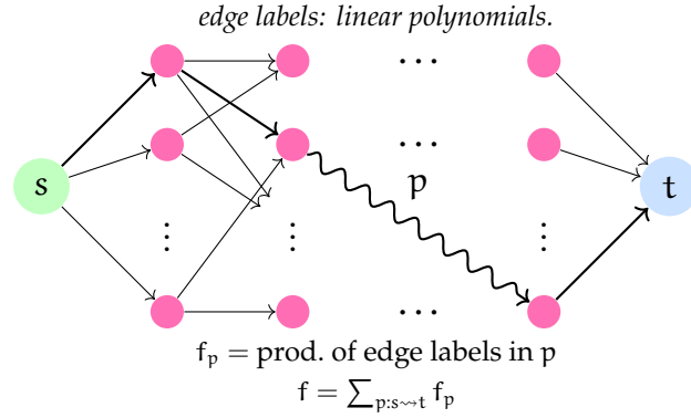
Figure 2.2: Algebraic Branching Program (ABP)
